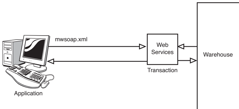
Figure 13.11 SOAP example.
