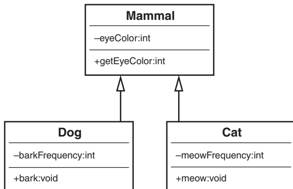
Figure 1.14 Mammal hierarchy.
