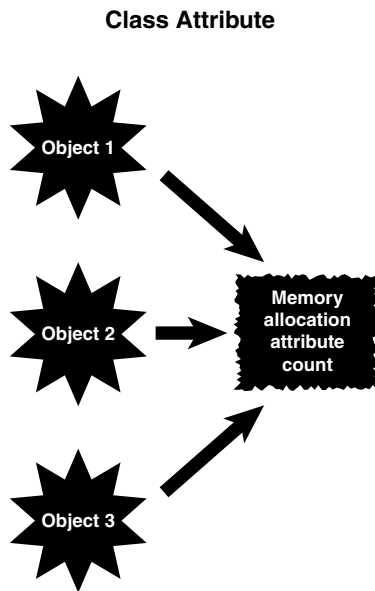
Figure 3.7 Class attributes.
