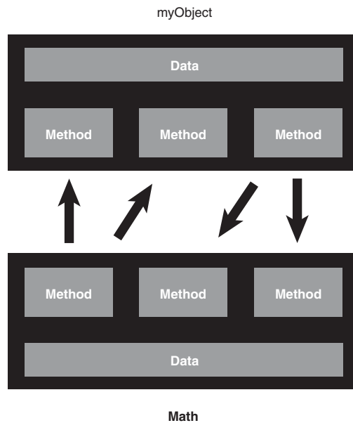
Figure 1.3 Object-to-object communication.
